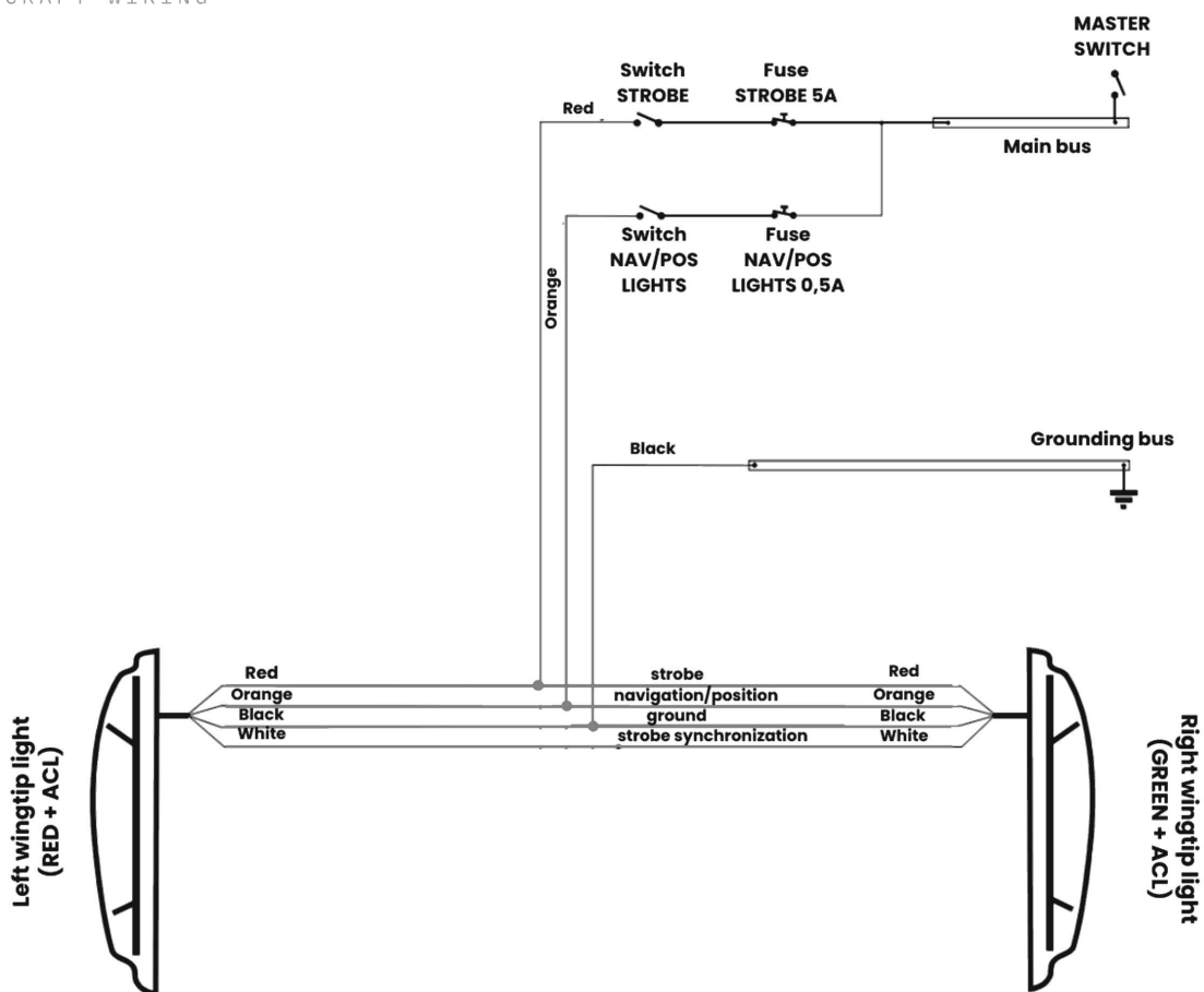
AIRCRAFT WIRING
