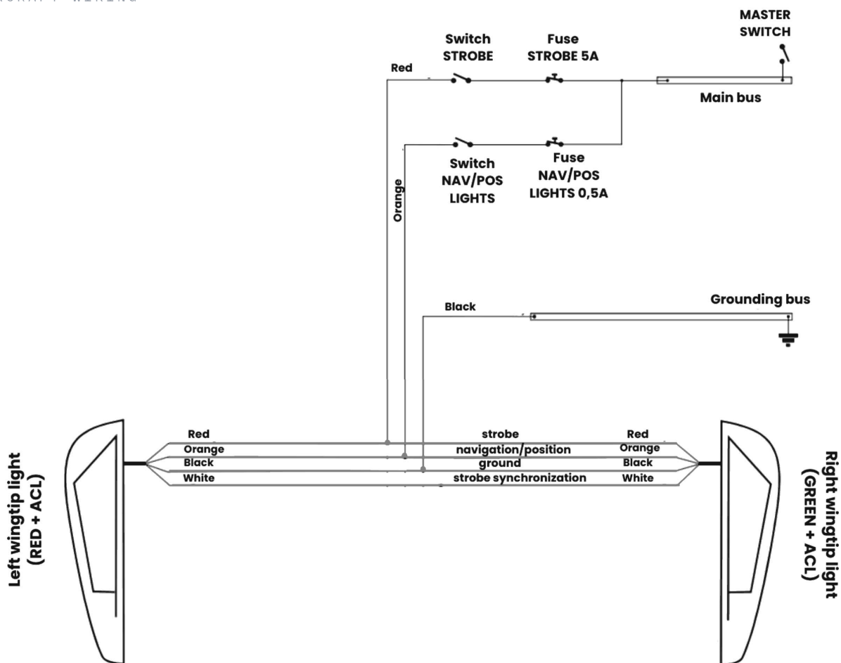
AIRCRAFT WIRING
