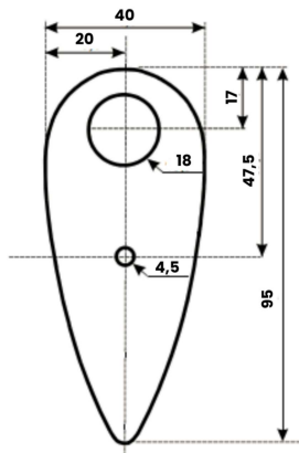
TOP VIEW · MOUNTING
